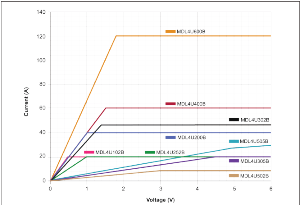
Typical minimum operating voltage at full scale current:
